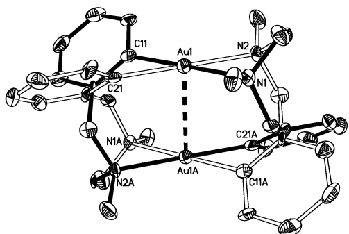
Figure 1. Disordered molecular structure of the compound [\text{Au}(\text{C}_6\text{H}_4\text{CH}_2\text{NMe}_2\text{-}2)]_2 (ORTEP drawing with 50% probability ellipsoids, H atoms omitted for clarity; sof 50/50). Selected bond lengths (Å) and angles (deg): Au1–N1 = 2.152(10), Au1–C11 = 2.042(15), Au1–N2 = 2.1371(2), Au1–C21 = 2.034(14), Au1⋯Au1A = 2.9176(5); N1–Au1–C11 = 179.7(5), N2–Au1–C21 = 179.4(4).
