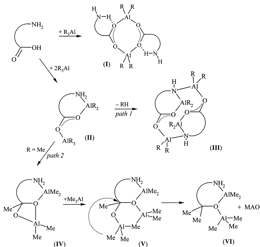
Scheme 2. Reaction Stages for the C-Alkylation of the Carboxylate Group by \text{AlMe}_3 Proposed by Mole 9
