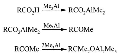
Scheme 2. Reaction Stages for the C-Alkylation of the Carboxylate Group by \text{AlMe}_3 Proposed by Mole 9
