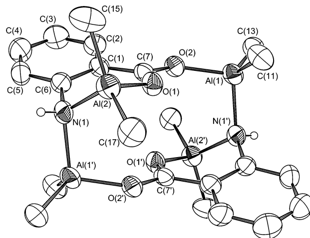
Figure 1. ORTEP view of [\text{Et}_2\text{Al}]_4[(\mu\text{-O}_2\text{C})\text{C}_6\text{H}_4\text{-}2\text{-}\mu\text{-NH}]_2 ( 4b ) with atom-numbering scheme. Thermal ellipsoids are shown at the 30% probability level. Methyl groups of the ethyl substituents are omitted for clarity.
