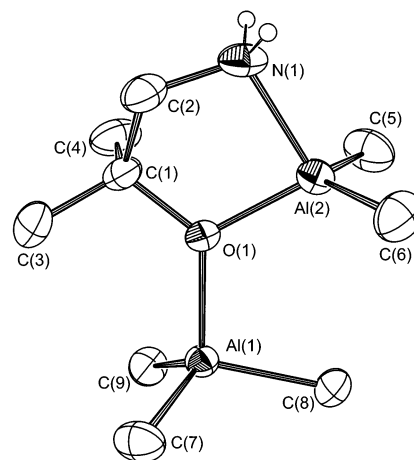
Figure 2. ORTEP view of \text{Me}_2\text{Al}[\text{OC}(\text{CH}_3)_2\text{CH}_2\text{NH}_2]\text{AlMe}_3 ( 7 ) with atom-numbering scheme. Thermal ellipsoids are shown at the 30% probability level. Hydrogen atoms (excluding amine hydrogens) are omitted for clarity.
