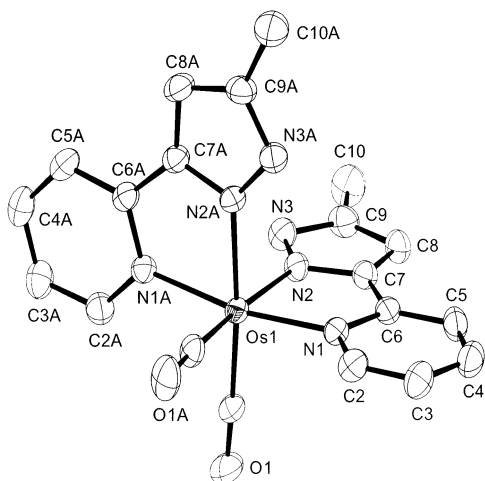
Figure 3. ORTEP diagram of complex 3 with thermal ellipsoids shown at 30% probability; the fluorine atoms of the \text{CF}_3 substituent on the pyrazolate fragments were removed for clarity.
