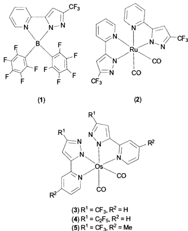
Figure 1. Structures of various B(III), Ru(II), and Os(II) complexes in this study.
