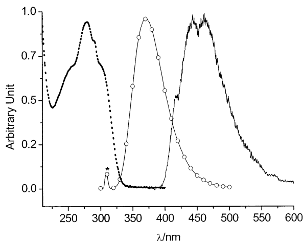
Figure 6. (a) Room-temperature UV-vis absorption (---) and fluorescence (—○—) spectra of pypz anionic species (pypzK) in CH 3 CN containing 1 M KOH. (b) Phosphorescence spectrum of pypz anion (—) in the 77 K solid (CH 3 CN) matrix acquired at a delay time of 1 μs. * denotes Raleigh scattering.
