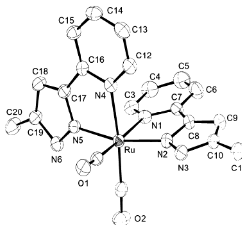
Figure 2. ORTEP diagram of complex 2 with thermal ellipsoids shown at 30% probability; the fluorine atoms of the \text{CF}_3 substituent on the pyrazolate fragments were removed for clarity.
