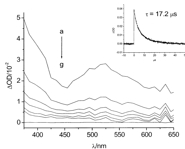
Figure 5. Temporal evolution of transient absorption spectra for complex 3 at a delay time of (a) 0.36, (b) 6, (c) 11.7, (d) 17.4, (e) 28.8, and (f) 40 \mu\text{s} in degassed \text{CH}_3\text{CN} ; (g) transient absorption spectrum of 3 acquired at a delay time of 2 \mu\text{s} in aerated \text{CH}_3\text{CN} . Inset: Decay profile of the transient signal at 550 nm (in degassed \text{CH}_3\text{CN} ). \lambda_{\text{ex}} : 355 nm.
