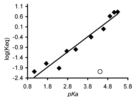
Figure 2. Plot of log K eq for the exchange reaction of 5d with Ar-BIAN as a function of the p K a of the aniline employed in the synthesis of Ar-BIAN. Data are given in Tables 1 and 2. The open circle corresponds to the data for 2,6- i Pr 2 C 6 H 3 -BIAN and was not included in the fitting.
