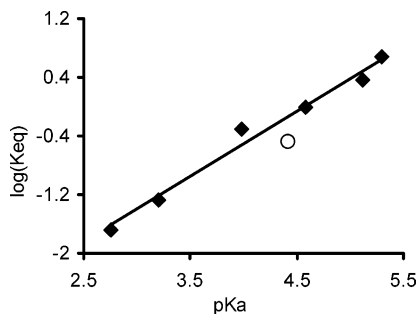
Figure 3. Plot of \log K_{\text{eq}} for the exchange reaction of 2d with Ar-BIAN as a function of the \text{p}K_{\text{a}} of the aniline employed in the synthesis of Ar-BIAN. Data are given in Tables 1 and 2. The open circle corresponds to the data for 2,6- i -Pr 2 C 6 H 3 -BIAN and was not included in the fitting.
