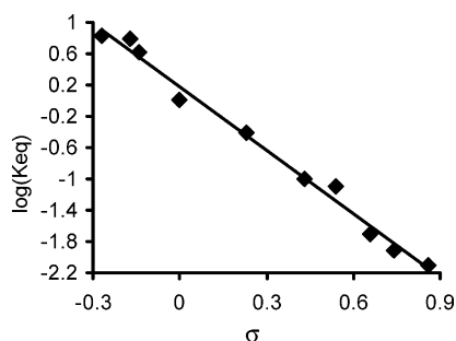
Figure 1. Plot of log K eq for the exchange reaction of 5d with Ar-BIAN as a function of the Hammett σ constants for the substituents on the aryl group of Ar-BIAN. Data are given in Tables 1 and 2.
