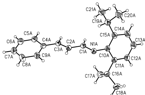
Figure 2. ORTEP drawing of the 1-aza-1,3-diene 1b (50% probability level) with the atom-labeling scheme.
