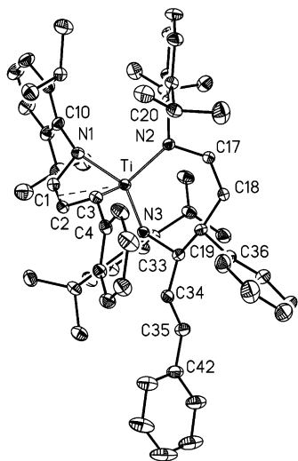
Figure 4. ORTEP drawing of complex 8 (50% probability level) with the atom-labeling scheme (hydrogen atoms have been omitted for clarity).
