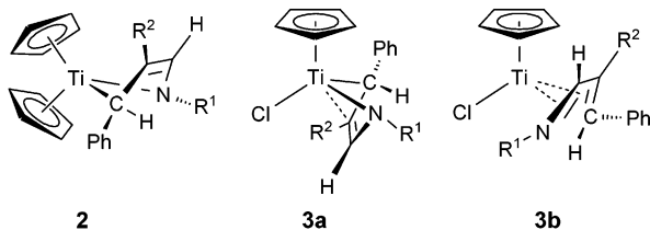
Chart 1. Structures of Cyclopentadienyltitanium 1-Aza-1,3-diene Complexes
