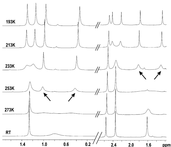
Figure 5. ^1\text{H} NMR spectra measured as a function of temperature for the complexes 9b and 9c in the methyl region. For the 3,5-di- tert -butylphenyl complex (left) the restricted rotation is clearly visible at 253 K, whereas for the 3,5-dimethylphenyl compound (right) the restricted rotation is recognized at 233 K; for 9c , the ca. 2.55 ppm resonance stems from a N -methyl group ( \text{CD}_2\text{Cl}_2 ).
