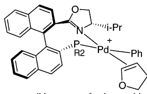
10 , one possible structure for the transition state
