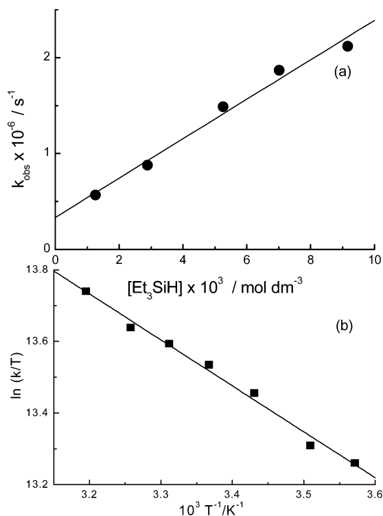
Figure 4. (a) Plot of k_{\text{obs}} versus [\text{Et}_3\text{SiH}] ( \lambda_{\text{exc}} = 308 nm, \lambda_{\text{mon}} = 390 nm). (b) Eyring plot showing the temperature variation of the second-order rate constant for reaction with \text{Et}_3\text{SiH} .
