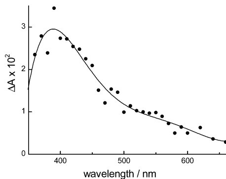
Figure 1. Point-by-point transient spectrum measured 100 ns after laser flash photolysis of Ru(eti)(CO)H 2 ( 1 ) in cyclohexane under 700 Torr of dihydrogen. The line is a fit to the points with a polynomial of order 6.
