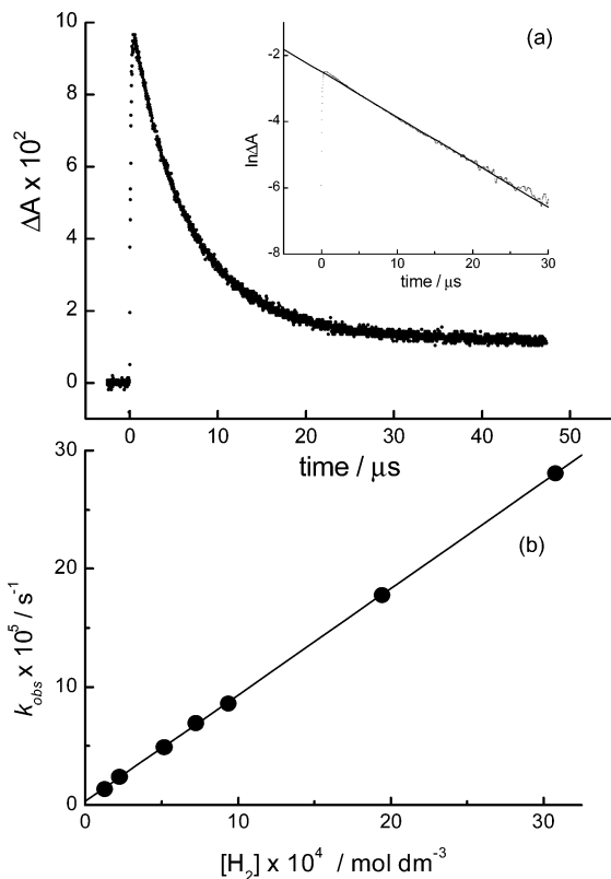
Figure 2. (a) Decay of the transient (monitoring wavelength, \lambda = 390 nm) generated upon laser flash photolysis (excitation wavelength, \lambda = 308 nm) of 1 in cyclohexane at 295 K under a partial pressure of 30 Torr of H 2 . The inset plot shows the fitting to pseudo-first-order behavior. (b) Plot of k_{\text{obs}} versus concentration of dissolved H 2 , yielding, from the slope, the second-order rate constant for reaction of the transient with added H 2 .
