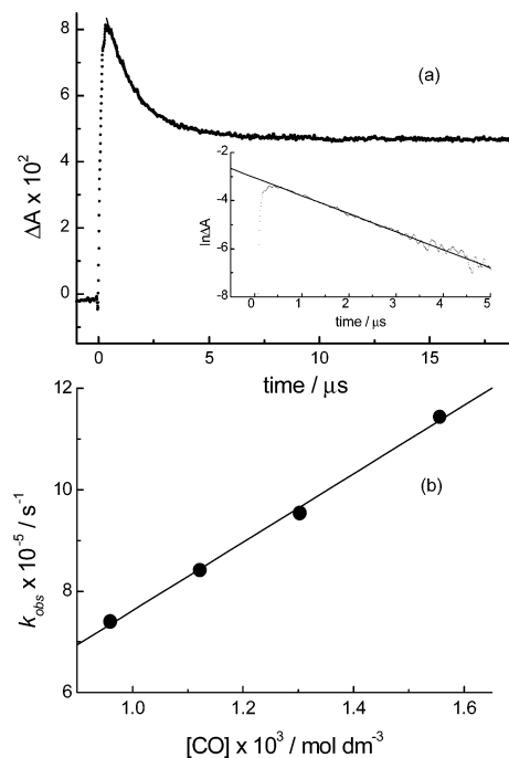
Figure 3. (a) Kinetic trace obtained upon flash photolysis of 1 in cyclohexane in the presence of CO ( 0.96 \times 10^{-3} mol dm -3 ). The inset plot shows the fitting to pseudo-first-order behavior. (b) Plot of k_{\text{obs}} versus [CO] ( \lambda_{\text{exc}} = 308 nm, \lambda_{\text{mon}} = 390 nm).
