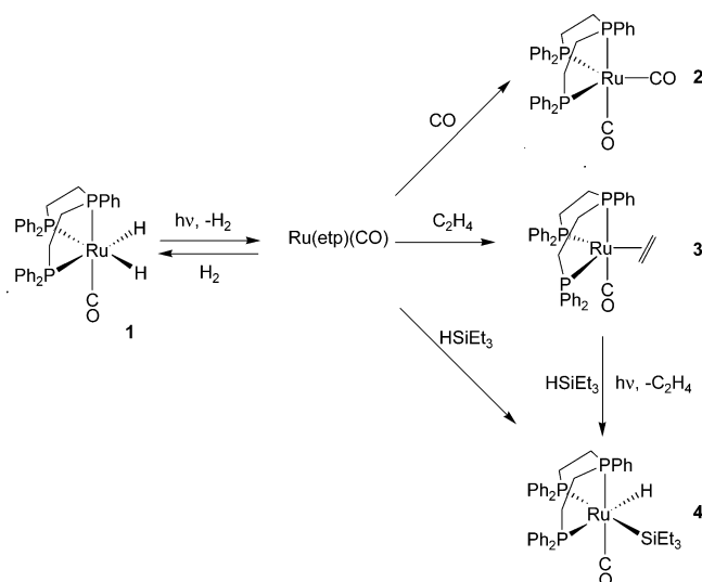
Scheme 1. Photochemical Reactions of Ru(eti)(CO)(H) 2 (1)
