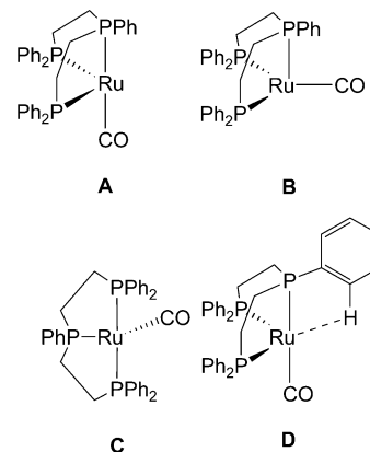
Scheme 2. Possible Structures for Ru(eti)(CO)
