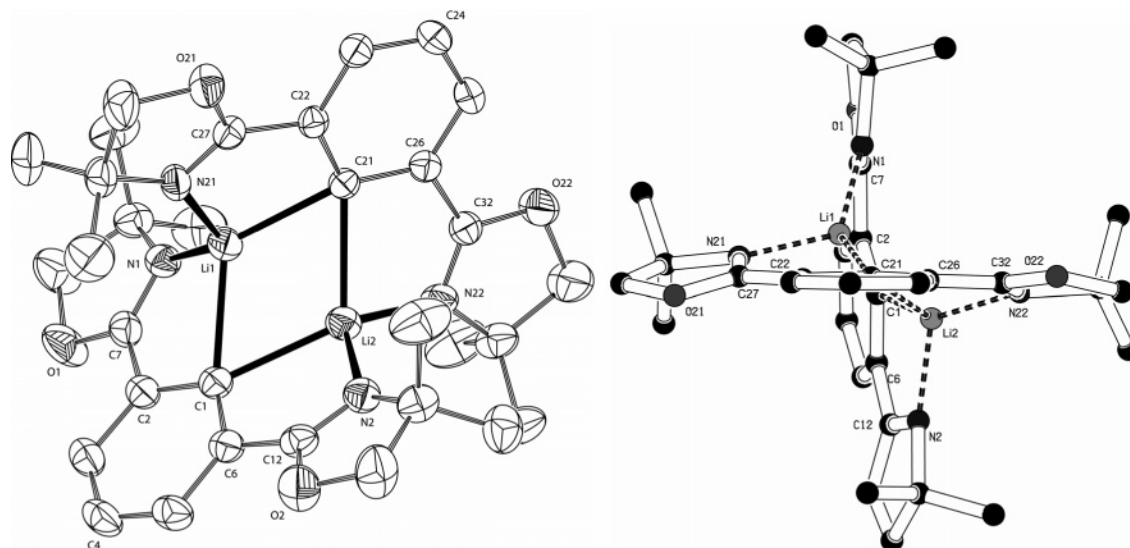
Figure 3. Top and side-on views of the crystal structure of [\text{Li}(\text{Me,Me-Phebox})]_2 . Hydrogen atoms have been omitted for clarity. Relevant bond distances (Å) and angles (deg): \text{C}(1)\text{--Li}(1) = 2.268(3) , \text{C}(1)\text{--Li}(2) = 2.289(3) , \text{C}(21)\text{--Li}(1) = 2.247(3) , \text{C}(21)\text{--Li}(2) = 2.299(3) , \text{Li}(1)\text{--N}(1) = 2.004(3) , \text{Li}(1)\text{--N}(21) = 1.987(3) , \text{Li}(2)\text{--N}(2) = 1.989(3) , \text{Li}(2)\text{--N}(22) = 2.006(3) ; \text{Li}(1)\text{--C}(1)\text{--Li}(2) = 61.61(10) , \text{Li}(1)\text{--C}(21)\text{--Li}(2) = 61.74(10) , \text{C}(1)\text{--Li}(1)\text{--C}(21) = 117.99(13) , \text{C}(1)\text{--Li}(1)\text{--N}(1) = 84.46(10) , \text{C}(1)\text{--Li}(1)\text{--N}(21) = 114.11(14) , \text{N}(1)\text{--Li}(1)\text{--N}(21) = 121.39(14) , \text{N}(21)\text{--Li}(1)\text{--C}(21) = 85.76(11) , \text{N}(1)\text{--Li}(1)\text{--C}(21) = 135.61(15) , \text{C}(1)\text{--Li}(2)\text{--C}(21) = 115.03(12) , \text{C}(1)\text{--Li}(2)\text{--N}(2) = 84.78(11) , \text{C}(1)\text{--Li}(2)\text{--N}(22) = 139.79(14) , \text{N}(2)\text{--Li}(2)\text{--N}(22) = 118.46(14) , \text{N}(22)\text{--Li}(2)\text{--C}(21) = 84.24(11) , \text{N}(2)\text{--Li}(2)\text{--C}(21) = 117.84(13) .
