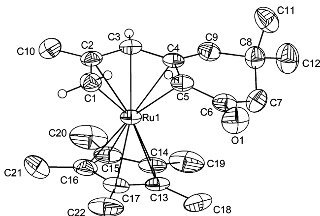
Figure 6. Perspective view of compound 18 . Most hydrogen atoms omitted for clarity.
