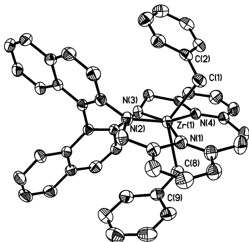
Figure 4. Thermal ellipsoid (50%) plot of [\text{MepyN}]\text{Zr}(\text{CH}_2\text{Ph})_2 . Hydrogen atoms are omitted for clarity.
