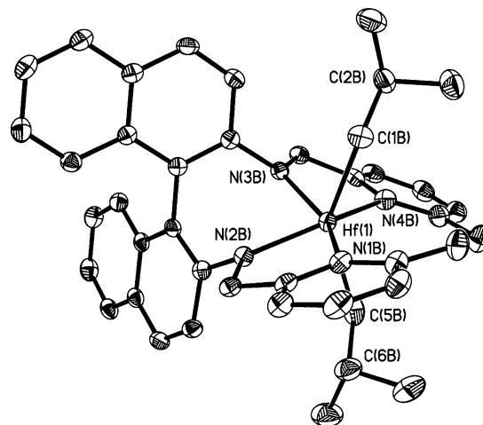
Figure 3. Thermal ellipsoid (50%) plot of [MepyN]Hf(CH 2 CHMe 2 ) 2 (one of two chemically equivalent molecules in the asymmetric unit). Hydrogen atoms are omitted for clarity.
