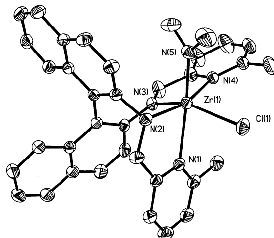
Figure 1. Thermal ellipsoid (50%) plot of [MepyN]Zr(NMe 2 )Cl. Hydrogen atoms are omitted for clarity.
