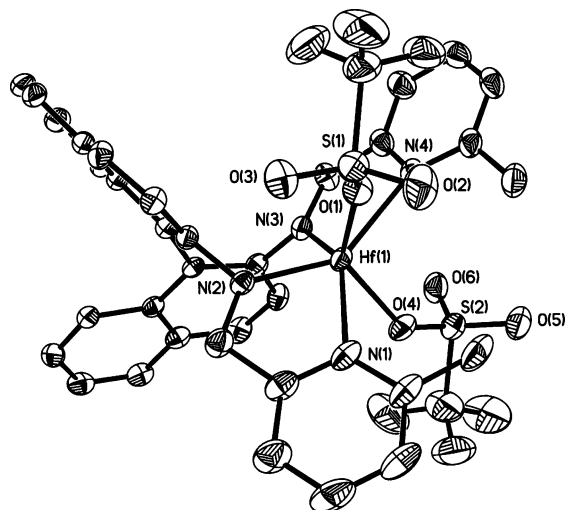
Figure 2. Thermal ellipsoid (50%) plot of [MepyN]Hf(OSO 2 CF 3 ) 2 . Hydrogen atoms are omitted for clarity.
