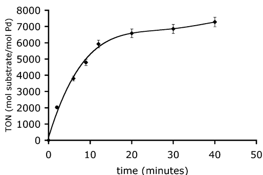
Figure 4. Conversion (TON) versus time plot for complex 17 . General conditions: Pd:substrate = 1:10173, [phenylacetylene] = 1.4 mmol/mL, 50 °C, 40 bar CO, solvent = MeOH.
