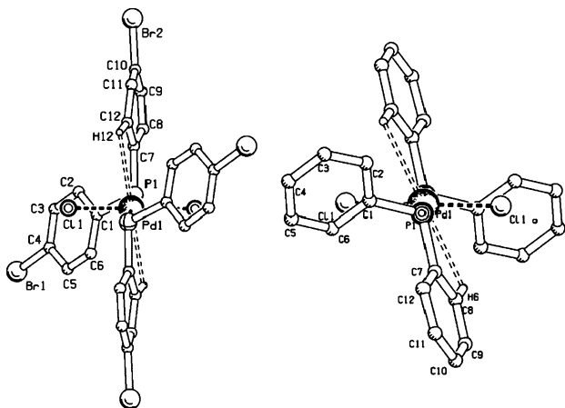
Figure 2. Crystal structure of 12 (left) and trans -[PdCl 2 (PPh 3 ) 2 ] (right), showing the tilting of one of the phenyl rings. For 12 the pyridyl ring and all hydrogen atoms not involved have been omitted; for trans -[PdCl 2 (PPh 3 ) 2 ] one of the phenyl rings and all hydrogen atoms not involved have been omitted.
