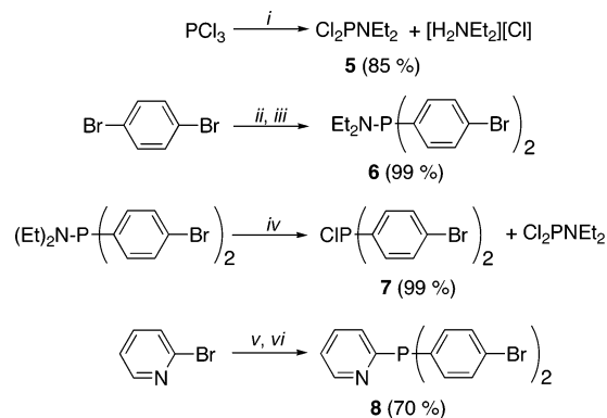
Scheme 1. Synthetic Route for 2-[Bis{4-(bromo)phenyl}phosphino]pyridine 8 a
