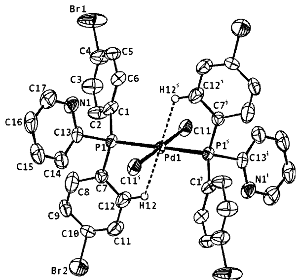
Figure 1. Displacement ellipsoid plot of 12 , drawn at the 50% probability level. All hydrogen atoms, except H(12) and H(12) i , have been omitted for clarity. Only one orientation of the disordered bromophenyl groups is shown. Symmetry operation i : -x, -y, -z .
