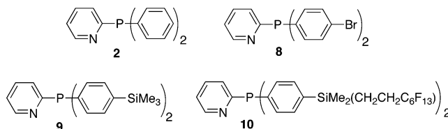
Scheme 1. Synthetic Route for 2-[Bis{4-(bromo)phenyl}phosphino]pyridine 8 a
