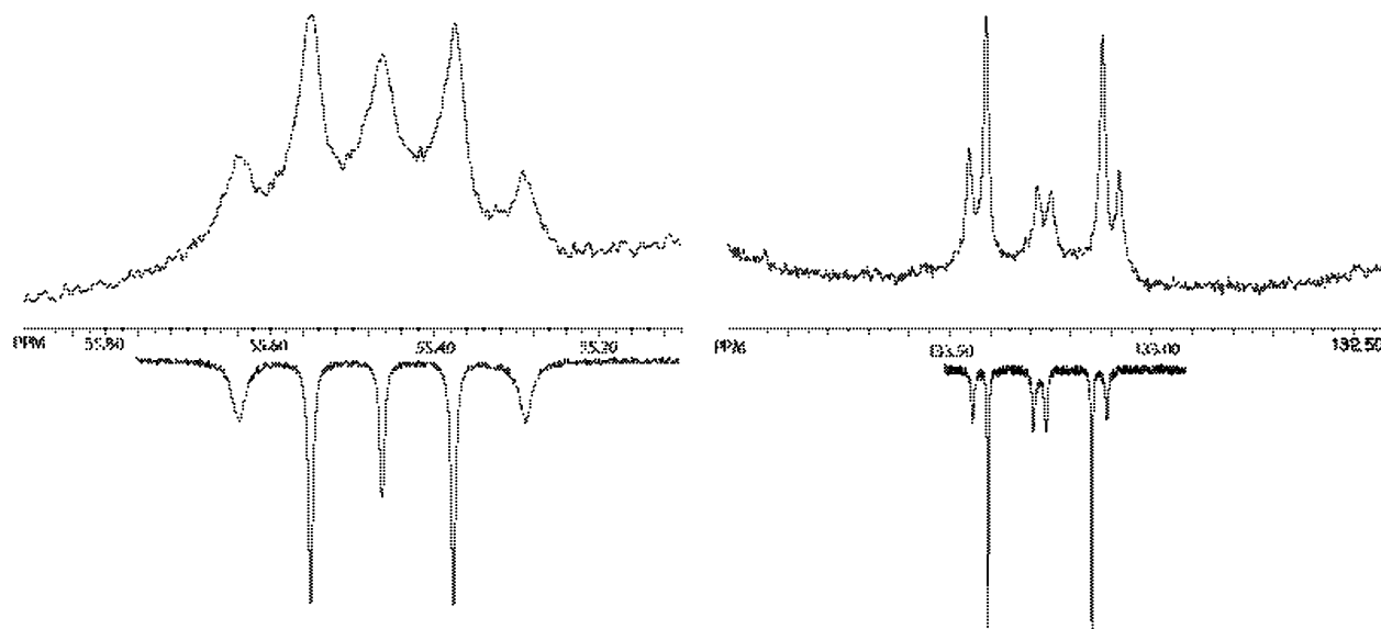
Figure 3. ^{13}\text{C}\{^1\text{H}\} NMR spectrum, alkene region (top left) and part of the aromatic region (top right) of complex 17 , in \text{CD}_2\text{Cl}_2 at -40^\circ\text{C} . Bottom left and right are simulations of these patterns.
