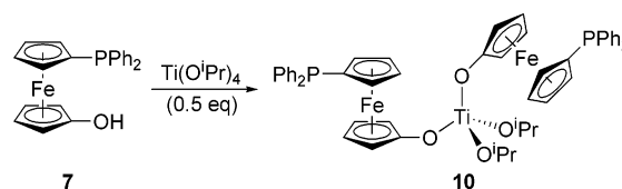
Scheme 5. Synthesis of Compound 10
