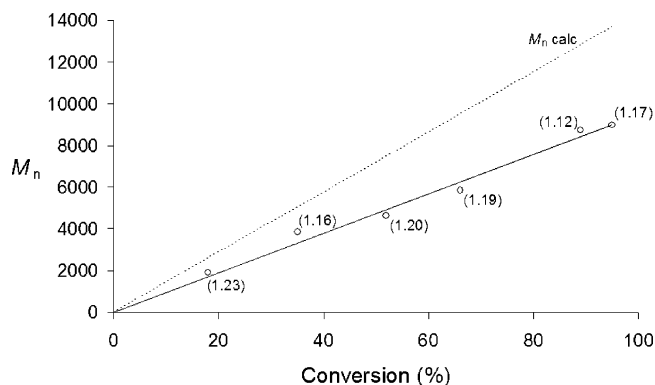
Figure 1. Plot of M_n vs monomer conversion for the polymerization of rac -LA using 10 (toluene, 70 °C, [LA]_0/[Ti] = 100 ) (polydispersities shown in parentheses).
