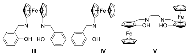
Scheme 2. Recent Examples of "Salen"-Type Compounds with Ferrocene Units Appended
