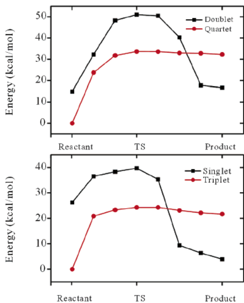
Figure 2. Calculated minimum-energy pathways of both high-spin and low-spin states of \text{Co}(\text{iPr-MeAMD})_2 and \text{Ni}(\text{iPr-MeAMD})_2 .
