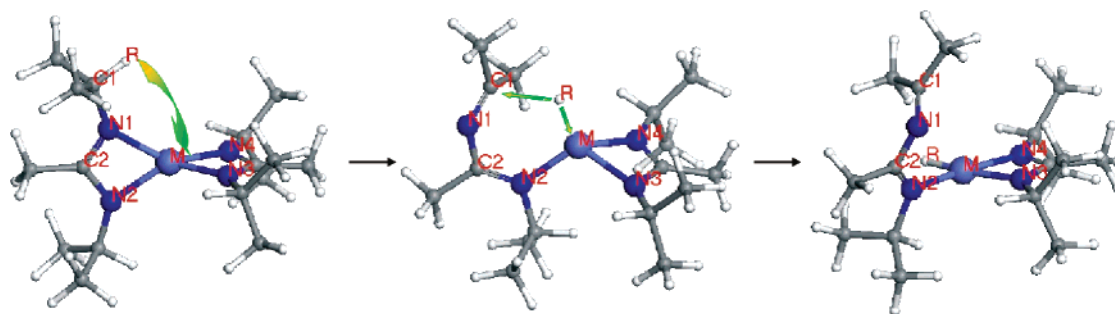
Figure 1. Structures of the reactant, transition state, and product: M = Ni, Co and R = H, CH 3 .
