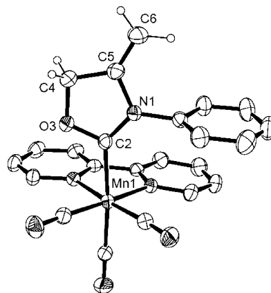
Figure 3. Molecular structure of 8a , shown with 30% thermal ellipsoids. Hydrogen atoms of the bipy ligand and phenyl substituent are omitted for clarity. Selected interatomic distances (Å) and angles (deg): Mn1–C2 = 2.042(3), N1–C2 = 1.335(4), C2–O3 = 1.340(3), O3–C4 = 1.464(4), C4–C5 = 1.496(4), C5–N1 = 1.438(4), C5–C6 = 1.319(5); Mn1–C2–N1 = 135.0(2), Mn1–C2–O3 = 116.5(2), N1–C2–O3 = 108.5(2), C2–O3–C4 = 111.5(2), O3–C4–C5 = 103.5(2), C4–C5–N1 = 103.3(2), C5–N1–C2 = 113.0(2).
