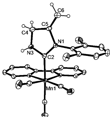
Figure 2. Molecular structure of 3b , shown with 30% thermal ellipsoids. Hydrogen atoms of the bipy ligand and 2,6-difluorophenyl substituent are omitted for clarity. Selected interatomic distances (Å) and angles (deg): Mn1–C2 = 2.068(3), N1–C2 = 1.375(3), C2–N3 = 1.338(3), N3–C4 = 1.458(3), C4–C5 = 1.481(4), C5–N1 = 1.437(3), C5–C6 = 1.350(4); Mn1–C2–N1 = 132.2(2), Mn1–C2–N3 = 122.6(2), N1–C2–N3 = 105.1(2), C2–N3–C4 = 114.9(2), N3–C4–C5 = 102.2(2), C4–C5–N1 = 104.6(2), C5–N1–C2 = 113.1(2).
