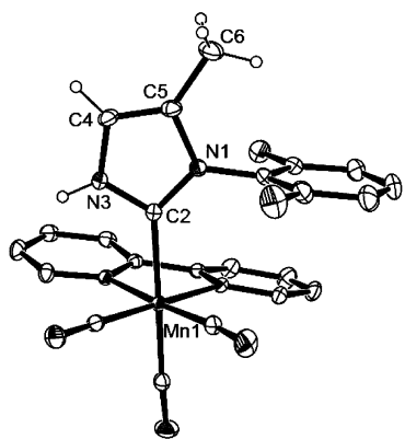
Figure 1. Molecular structure of 4b , shown with 30% thermal ellipsoids. Hydrogen atoms of the bipy ligand and 2,6-difluorophenyl substituent are omitted for clarity. Selected interatomic distances (Å) and angles (deg): Mn1–C2 = 2.078(2), N1–C2 = 1.377(3), C2–N3 = 1.354(3), N3–C4 = 1.398(3), C4–C5 = 1.354(3), C5–N1 = 1.417(3), C5–C6 = 1.501(3); Mn1–C2–N1 = 133.3(1), Mn1–C2–N3 = 124.3(2), N1–C2–N3 = 102.3(2), C2–N3–C4 = 113.3(2), N3–C4–C5 = 106.7(2), C4–C5–N1 = 105.2(2), C5–N1–C2 = 112.5(2).
