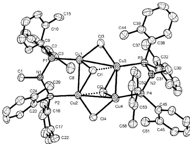
Figure 6. Crystal structure of [(\text{Ar}_2\text{PN}(\text{Me})\text{PAR}_2)\text{Cu}_2\text{Cl}_2]_2 {Ar = 2- \text{C}_6\text{H}_4(\text{Me}) } ( 23 ) (hydrogens and solvent omitted for clarity).
