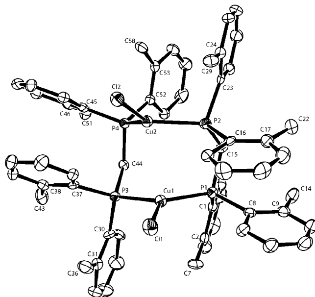
Figure 4. Crystal structure of [(\text{Ar}_2\text{PCH}_2\text{PAR}_2)\text{CuCl}]_2 {Ar = 2- \text{C}_6\text{H}_4(\text{Me}) } ( 14 ) (hydrogens and solvent omitted for clarity).
