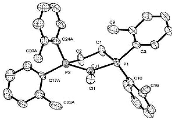
Figure 5. Crystal structure of [(\text{Ar}_2\text{PCH}_2\text{CH}_2\text{PAR}_2)\text{CuCl}] {Ar = 2- \text{C}_6\text{H}_4(\text{Me}) } ( 17 ) (hydrogens omitted for clarity).
