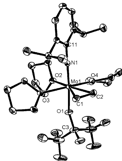
Figure 6. Thermal ellipsoid (50%) rendering of \{\text{Mo}(\text{NAr})(\text{C}_2\text{H}_4)[\text{OCMe}(\text{CF}_3)_2](\text{THF})_3\}\text{BARF}_4 ( 6 ). Hydrogen atoms, a minor disorder, a disordered pentane, and the anion are removed for clarity. Selected bond distances ( \text{\AA} ) and angles (deg): \text{Mo1}-\text{C1} = 2.213(2) ; \text{Mo1}-\text{C2} = 2.220(2) ; \text{Mo1}-\text{N1} = 1.7558(19) ; \text{Mo1}-\text{O1} = 2.0196(17) ; \text{Mo1}-\text{O2} = 2.2499(16) ; \text{Mo1}-\text{O3} = 2.2013(17) ; \text{Mo1}-\text{O4} = 2.2051(17) ; \text{C1}-\text{C2} = 1.408(4) ; \text{Mo1}-\text{C1}-\text{C2} = 71.76(14) ; \text{Mo1}-\text{C2}-\text{C1} = 71.20(14) ; \text{Mo1}-\text{N1}-\text{C11} = 178.17(16) ; \text{Mo1}-\text{O1}-\text{C3} = 157.7(2) ; \text{N1}-\text{Mo1}-\text{O1} = 175.71(8) .
