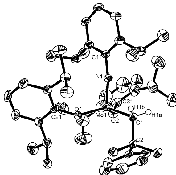
Figure 5. Thermal ellipsoid (50%) rendering of the well-behaved molecule of the structure of [\text{Mo}(\text{NAr})(\text{CH}_2\text{CMe}_2\text{Ph})(\text{O}-2,6-i\text{-Pr}_2\text{C}_6\text{H}_3)_2]\text{BARF}_4 ( 4 ). Hydrogen atoms (except for the alkyl's \alpha protons) and the anion are removed for clarity. Selected bond distances ( \text{\AA} ) and angles (deg): \text{Mo1}-\text{C1} = 2.113(4) ; \text{Mo1}-\text{N1} = 1.699(3) ; \text{Mo1}-\text{O1} = 1.840(3) ; \text{Mo1}-\text{O2} = 1.843(3) ; \text{Mo1}-\text{C1}-\text{C2} = 110.1(3) ; \text{Mo1}-\text{N1}-\text{C11} = 170.6(3) ; \text{Mo1}-\text{O1}-\text{C21} = 145.1(3) ; \text{Mo1}-\text{O2}-\text{C31} = 139.4(3) .
