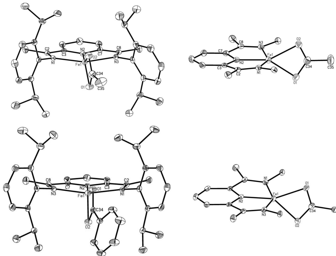
Figure 3. Molecular structure of 1-OAc (top) and 1-OBz (bottom) at 30% probability ellipsoids. View of the core of the molecules (right). Hydrogen atoms are omitted for clarity.
