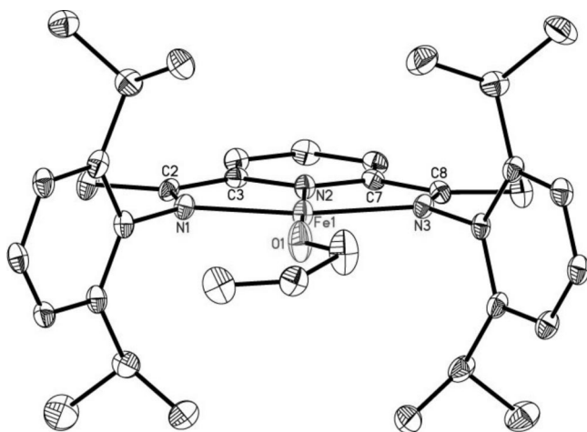
Figure 2. Molecular structure of 1-OCH 2 CH=CH 2 at 30% probability ellipsoids. Hydrogen atoms are omitted for clarity.
