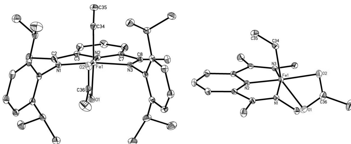
Figure 5. Molecular structure of 1-(OAc)(Vinyl) at 30% probability ellipsoids (left). Side view of the core of the molecule (right). Hydrogen atoms are omitted for clarity.
