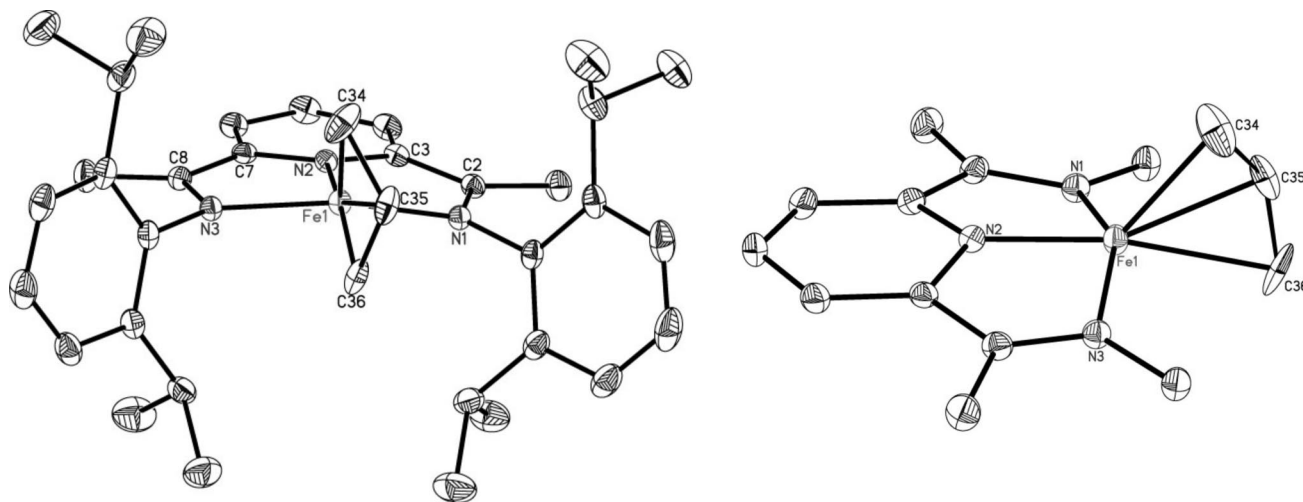
Figure 4. Molecular structure of 1-Allyl at 30% probability ellipsoids. Hydrogen atoms are omitted for clarity. Core of the molecule presented on the right.
