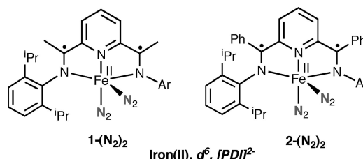
Figure 1. Bis(dinitrogen) iron complexes bearing redox active bis(imino)pyridine ligands.
