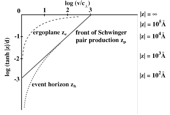
FIG. 3. Locations of the horizons, the ergoplanes, and the boundaries of the region of pair production by the electric field, as a function of the velocity v of the soliton.
