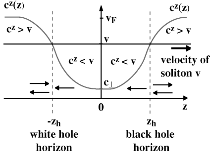
FIG. 2. The speed of light in the z direction in the superfluid frame c^z(z) . Quasiparticles in the region -z_h < z < z_h , where the speed of light is less than the velocity v of the soliton, cannot propagate to the right in the frame of the moving texture (the arrows show the possible directions of quasiparticle motion in the z direction). This region is bounded by the black and white hole horizons.
