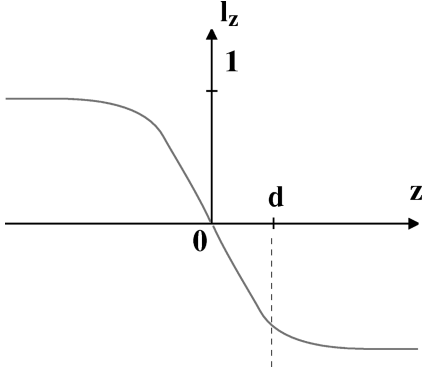
FIG. 1. Profile of the z projection of the vector \vec{l} across the splay soliton wall in a superfluid {}^3\text{He-A} . This soliton is topologically stable and can propagate in the liquid without destruction.
