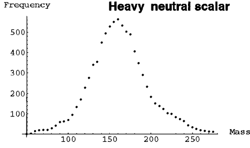
FIG. 5. Frequency distribution of the heavy neutral scalar mass (in GeV) for the baryon preserving cases.
