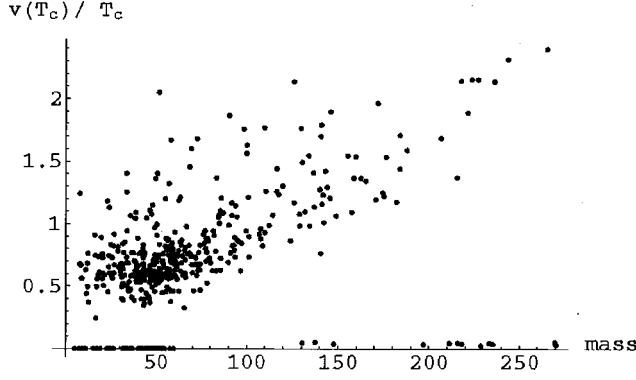
FIG. 1. v(T_c)/T_c ratio vs the lightest scalar mass (in GeV).
