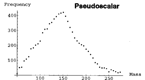
FIG. 4. Frequency distribution of the pseudoscalar mass (in GeV) for the baryon preserving cases.
