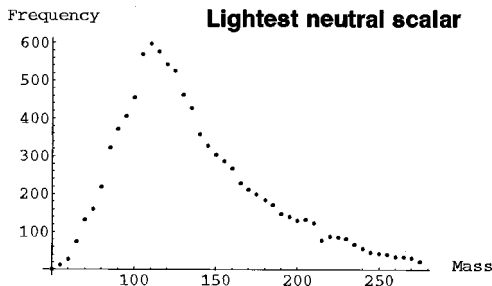
FIG. 2. Frequency distribution of the lightest neutral scalar mass (in GeV) for the baryon preserving cases.
