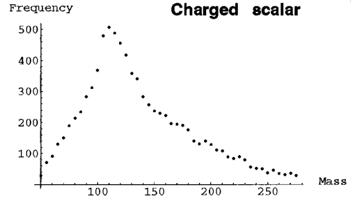
FIG. 3. Frequency distribution of the charged scalar mass (in GeV) for the baryon preserving cases.
