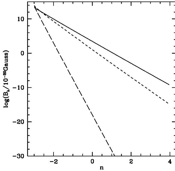
FIG. 2. We show the nucleosynthesis limit on B_\lambda (solid line) as function of the spectral index, n together with the limit from gravity waves if the primordial field is produced at the electroweak transition (short-dashed) or during inflation (long-dashed) for \lambda = 0.1 \text{ h}^{-1} \text{ Mpc} \approx 10^{13} \text{ sec} .
