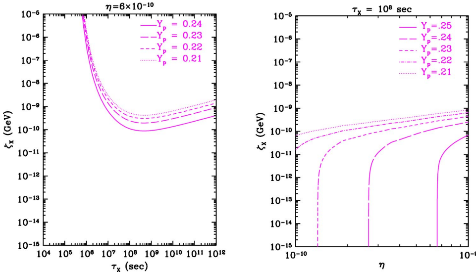
FIG. 1. (Color online) Contours of the {}^4\text{He} mass fraction Y_p (a) in the (\zeta_X, \tau_X) plane, for \eta_{10}=6 , and (b) in the (\zeta_X, \eta) plane, for \tau_X=10^8 s. See the text for discussion.
