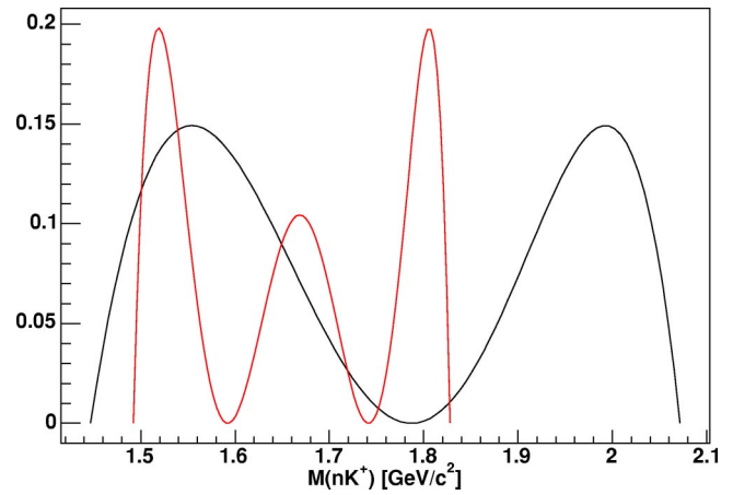
FIG. 2. The m_{KN} mass distribution for a fixed m_{K\bar{K}N} mass of 2.6 \text{ GeV}/c^2 . The two-peaked curve assumes m_{K\bar{K}} = m(a_2) with |Y_2^{\pm 1}|^2 and the three-peaked curve assumes m_{K\bar{K}} = m(\rho_3) - \Gamma_\rho/2 with |Y_3^{\pm 1}|^2 for the decay angular distribution.
