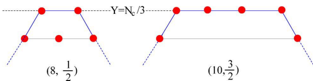
FIG. 3. Nonexotic ( X=0 ) multiplets that can be composed of N_c quarks.
