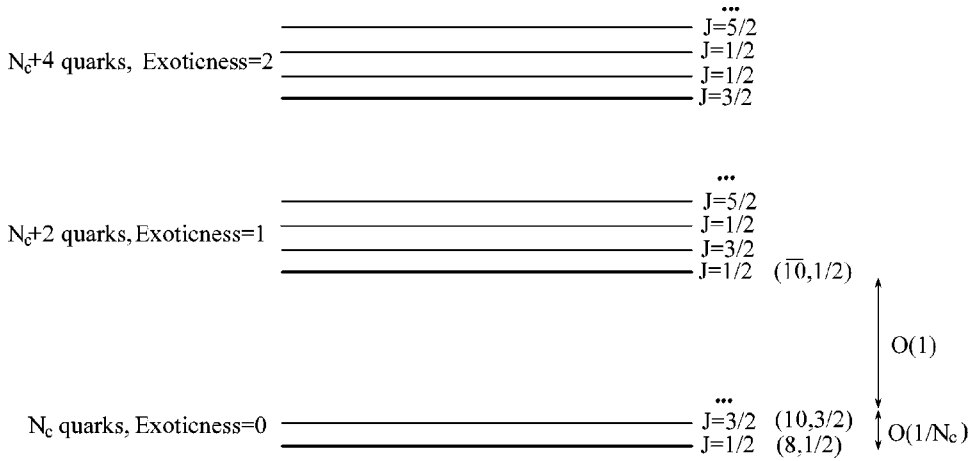
FIG. 2. Rotational excitations form a sequence of bands.
