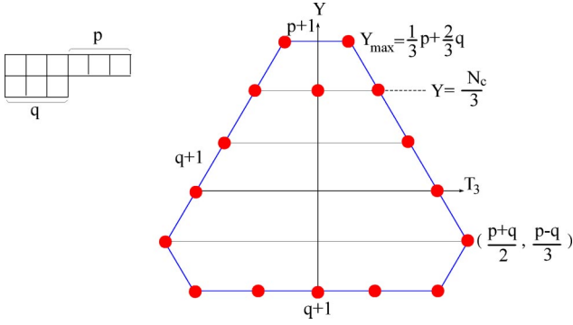
FIG. 1. A weight diagram of a generic SU(3) representation in the (T_3, Y) plane.
