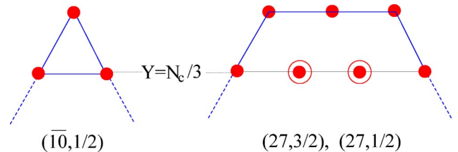
FIG. 4. Exotic ( X=1 ) multiplets that can be composed of N_c quarks and one extra pair.
