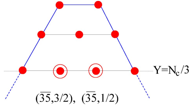
FIG. 5. Two lowest exotic ( X=2 ) multiplets that can be composed of N_c quarks and two extra pairs.
