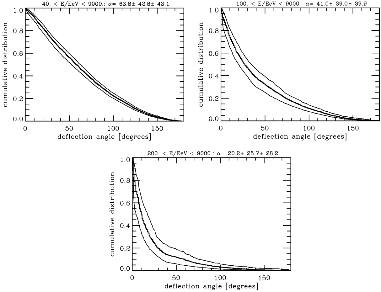
FIG. 6. The cumulative distribution of UHECR deflection angles with respect to the line of sight to the sources larger than \alpha , averaged over 24 realizations for scenario 6 in Table I. Shown are the distributions (middle, histogram) and 1\text{-}\sigma variations (upper and lower curves) above 4 \times 10^{19} eV (upper left panel), above 10^{20} eV (upper right panel), and above 2 \times 10^{20} eV (lower panel). Also given on top of the figures average and variances of the distributions.
