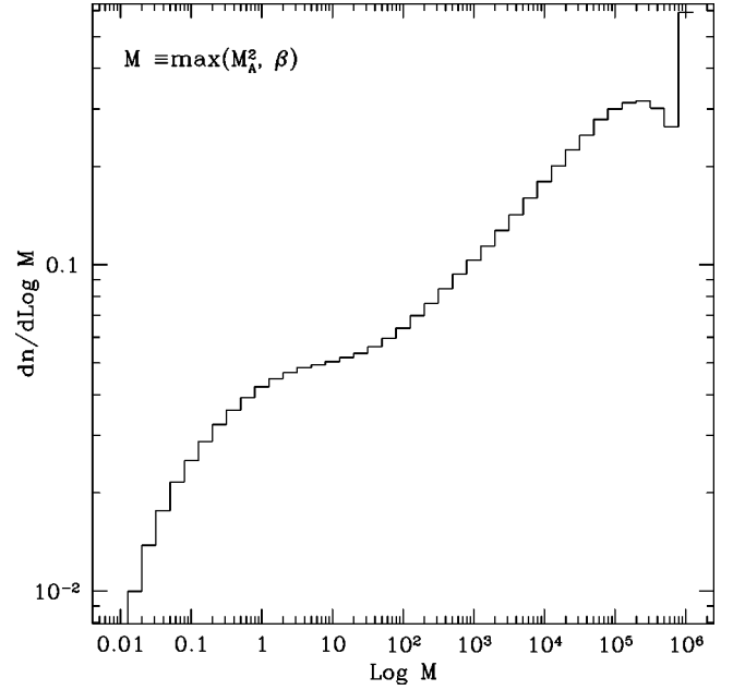
FIG. 1. Distribution of the number of cells n as a function of maximum M of the Alfvén Mach number and the plasma beta parameter.
