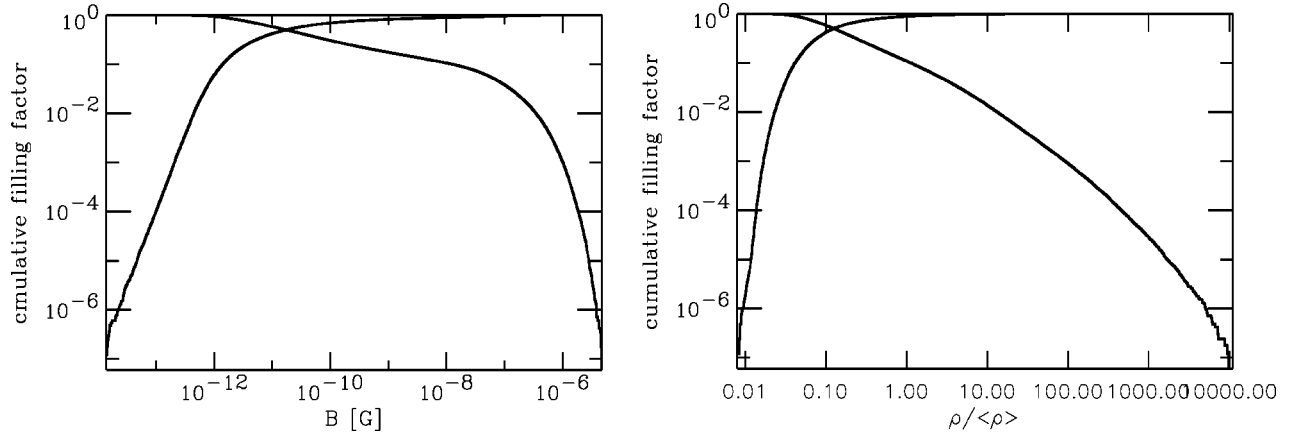
FIG. 2. The cumulative filling factors for EGMF strength, (left panel) baryon density (right panel, in units of average baryon density) above (decreasing curves) and below (increasing curves) a given threshold, as a function of that threshold.
