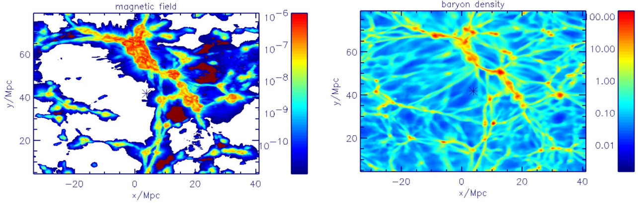
FIG. 4. Same as Fig. 3, but for an observer situated in a small void where the EGMF strength is \approx 10^{-11} G.
