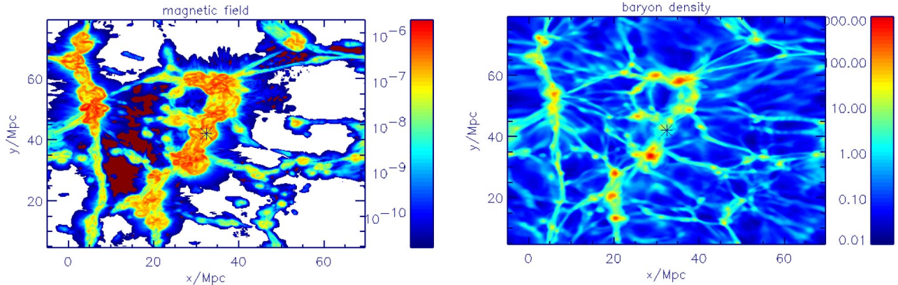
FIG. 3. Log-scale two-dimensional cut through magnetic field total strength in Gauss (color scale in Gauss, left panel) and baryon density in units of average baryon density (color scale, right panel). The observer is in the center of the figures and is marked by a star. The EGMF strength at the observer is \approx 0.1 \mu\text{G} . Note that both panels correspond to the same cuts through the full large scale simulation box.
