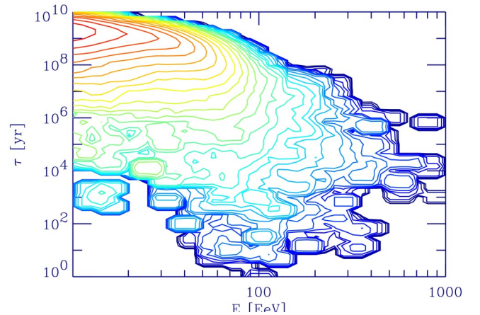
FIG. 5. The distribution of UHECR detection energy E and delay time \tau with respect to straight line propagation, for scenario 6 in Table I, averaged over 26 realizations of 10^4 simulated trajectories above 10^{19} eV each.
