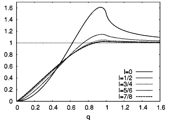
FIG. 8. The behavior of the function D_l for different values of l .
