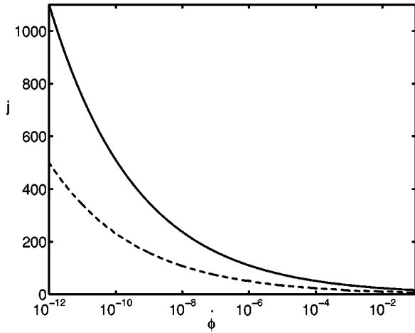
FIG. 2. Analytic results for HAM quantization with l=3/4 and initial conditions \phi_i=0 and \dot{\phi}_i>0 . The solid line corresponds to the case where the turning point of the inflaton is at \phi=3/l_{\text{Pl}}^{-1} . Sufficient inflation to solve the horizon problem arises in the region above this line. The kinetic bound is satisfied in the region below the dashed line. The two regions do not overlap.
