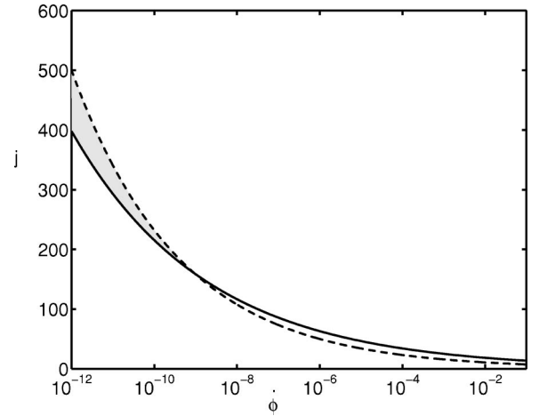
FIG. 4. Analytic results for FRIED quantization with l=3/4 and initial conditions \phi_i=0 and \dot{\phi}_i>0 . The horizon problem is solved in the region above the solid line and the kinetic bound is satisfied below the dashed line. The shaded area represents the region of parameter space that leads to successful inflation for this set of initial conditions.
