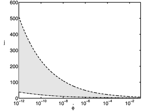
FIG. 7. Numerical results for FRIED quantization with l=3/4 , where the initial value of the inflaton is determined by imposing the uncertainty principle (27). The horizon problem is solved for all values of j and \dot{\phi}_i covered in the figure. The conditions for successful inflation are therefore limited only by the requirement that the classical phase corresponds to energy scales below the Planck scale. Successful inflation arises in the shaded region.
