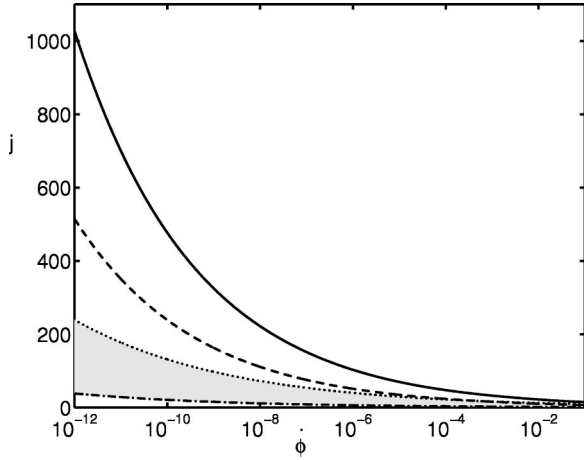
FIG. 6. Numerical results for HAM quantization with l=3/4 , where the initial value of the inflaton is determined by imposing the uncertainty principle (27). The horizon problem is solved in regions above the solid line and below the dotted line. The region below the dashed line satisfies the kinetic bound. The potential energy of the field exceeds the Planck scale below the dot-dashed line. Successful inflation is possible in the shaded region.
