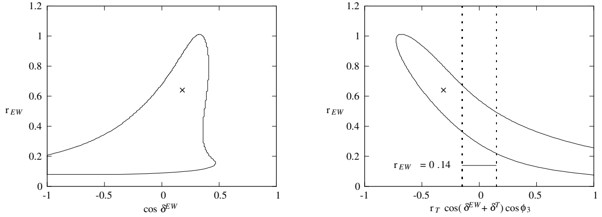
FIG. 1. The allowed region on (r_{EW}, \cos \delta^{EW}) and [r_{EW}, r_T \cos(\delta^{EW} + \delta^T) \cos \phi_3] plane at 1\sigma level varying the magnitude of r_T \cos(\delta^{EW} + \delta^T) \cos \phi_3 up to 1. The dashed line shows the bound of r_T \cos(\delta^{EW} + \delta^T) \cos \phi_3 for r_T = 0.2 and \phi_3 = 40^\circ .
