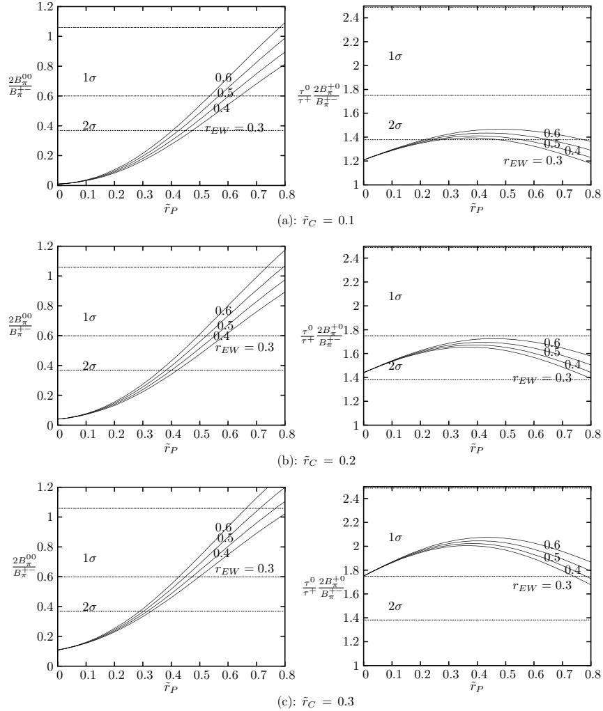
FIG. 5. \frac{2B_\pi^{00}}{B_\pi^+} and \frac{\tau^0 2B_\pi^{+0}}{B_\pi^+} as the functions of \tilde{r}_P at (a) \tilde{r}_C = 0.1 , (b) \tilde{r}_C = 0.2 and (c) \tilde{r}_C = 0.3 .
