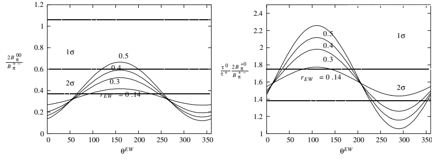
FIG. 9. \frac{2B^0_0}{B^+\pi^-} and \frac{\tau^0}{\tau^+} \frac{2B^+_0}{B^+\pi^-} as the function of \theta^{EW} at \tilde{r}_C = 0.2 , \omega = 0^\circ and \theta^P = 0^\circ . The gluonic penguin contribution \tilde{r}_P is 0.45, which is almost 1.5 times as large as the usual estimation in the SM.
