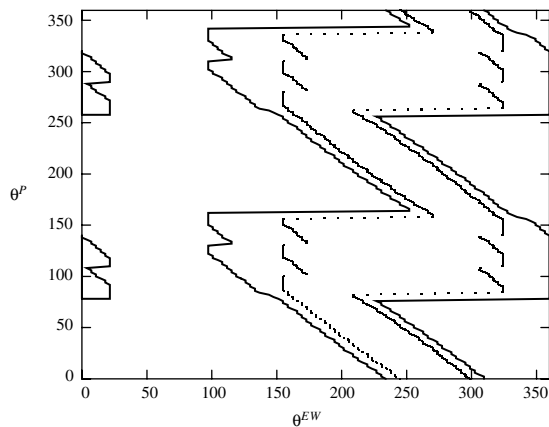
FIG. 8. The lines show the allowed region for \theta^{EW} and \theta^P satisfying the data of R_c - R_n and S a 1\sigma level. The solid line shows the case of r_{EW} = 0.40 and the dashed lines is r_{EW} = 0.30 at \omega = 0^\circ and r_T = 0.2 under constraint -0.123 < A_{CP}^{+-} < -0.067 and 40^\circ < \phi_3 < 80^\circ .
