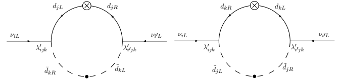
FIG. 1. Feynman diagrams representing the squark-quark loop contribution to the Majorana neutrino mass.
