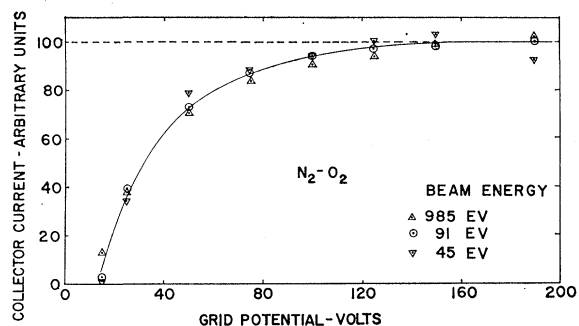
FIG. 1. N_2-O_2 collector current saturation curves.
