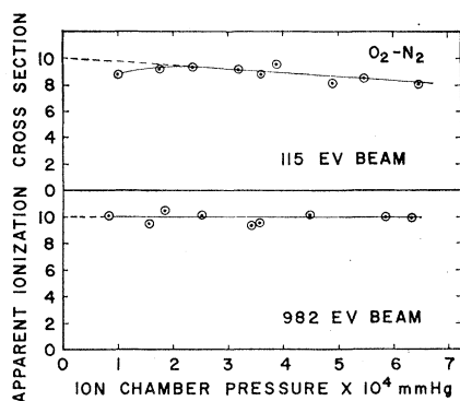
FIG. 8. O_2-N_2 pressure saturation curves.
