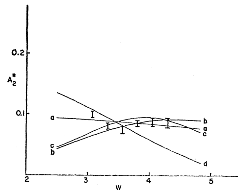
FIG. 3. Plots of A_2^* vs beta energy for the following matrix element parameter sets: (a) \zeta_1=2, u = -0.53, x = -0.4 ; (b) \zeta_1=2, u = 0.22, x = 1.55 ; (c) \zeta_1=2, u = 0.93, x = 0.9 ; and (d) \zeta_1=2, u = 0.38, x = -0.57 . Experimental values of A_2^* are also shown.
