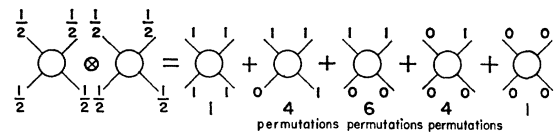
FIG. 3. Decomposition of direct products of spin- \frac{1}{2} basis functions.
