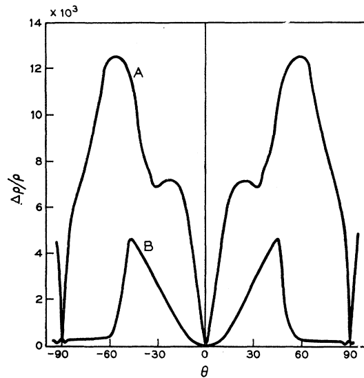
FIG. 3. Magnetoresistance rotation curves for zinc at 4.2°K, H=18\text{kg} , J\parallel[11\bar{2}0] . Curve A: transverse rotation, H\parallel[10\bar{1}0] at \theta=0^\circ . Curve B: Longitudinal rotation, H\parallel J at \theta=0^\circ , H\parallel[0001] at \theta=90^\circ .
