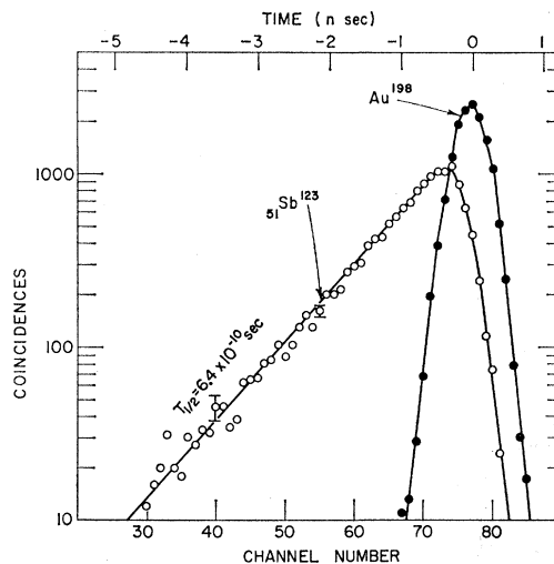
FIG. 5. Time spectrum of \beta - e coincidences in the decay of Sn 123 to Sb 123 .
