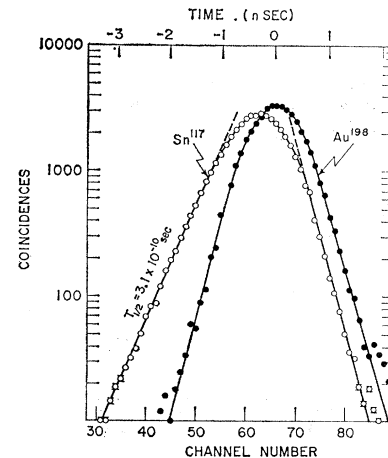
FIG. 2. Time spectra of e - e coincidences in the decay of Sn 117m . A "prompt" time distribution from \beta - \gamma coincidences in Au 198 decay is shown.
