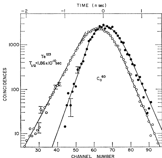
FIG. 4. Time spectrum of e - e coincidences in the decay of Te 123m . A prompt spectrum of e - \gamma coincidences from Co 60 is shown for comparison.
