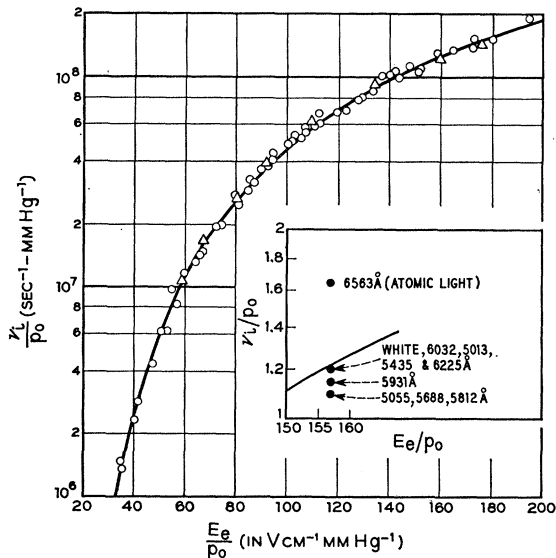
FIG. 3. Plot of \nu_i/p vs E_e/p_0 for \nu_c = 4.8 \times 10^9 p_0 ; \circ , line radiation and white light; \triangle , continuum radiation; solid curve is calculated from measurements of Rose.
