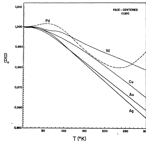
FIG. 11. The bulk moduli, normalized to their respective 0°K values, for certain of the face-centered cubic transition metals and for the noble metals.
