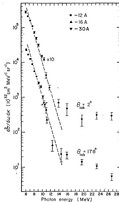
Fig. 4. Low-energy photon spectra from 185-MeV protons on aluminum, at 2 and 178 deg from the proton beam. The cross sections for the 2-deg spectrum have been increased a factor of 10 to separate the curves, and the dashed straight lines represent the same cross section for the two spectra. These spectra have not been corrected for spectrometer line shape; this correction would slightly increase the cross section at the lowest photon energies.
