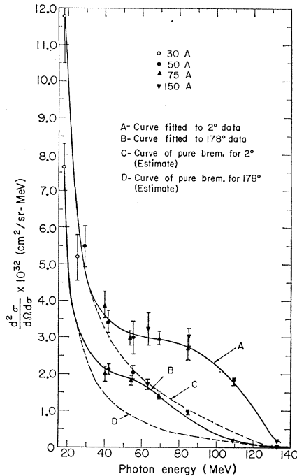
FIG. 5. Photon emission from 185-MeV protons on beryllium, at 2 and 178 deg from the proton beam. (A) Curve fitted to 2-deg data; (B) curve fitted to 178-deg data; (C) estimated curve for pure bremsstrahlung at 2 deg; (D) estimated curve for pure bremsstrahlung at 178 deg. (See text, Sec. III B for discussion of these curves.)
