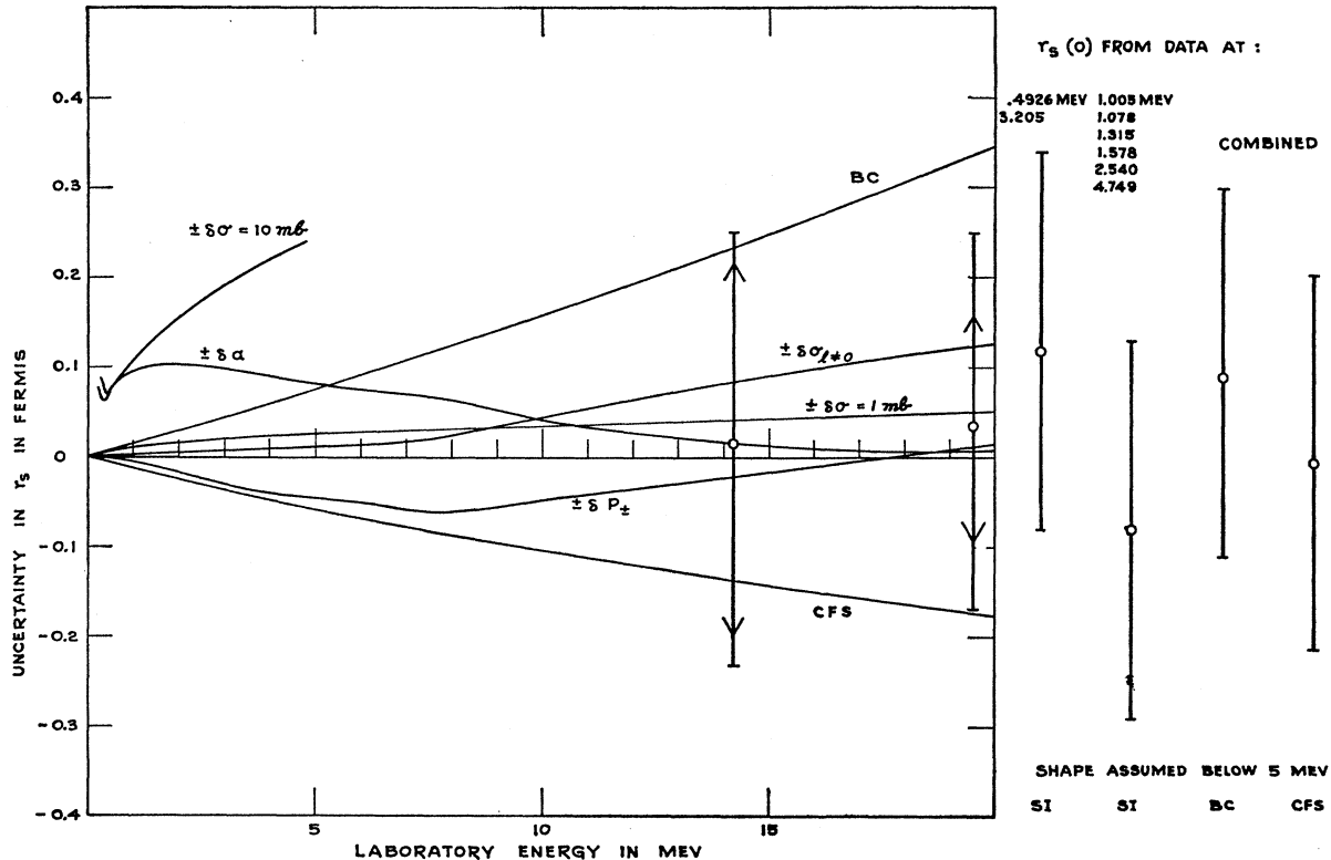
FIG. 2. Contributions to the uncertainty in the value of r_s computed from total cross-section measurements at a single energy: \pm\delta a due to uncertainty in the scattering lengths, \pm\delta\sigma_{l\neq 0} due to the scattering in other angular momentum states, \pm\delta P_l due to the triplet S shape dependence as estimated by the CFS formula, \pm\delta\sigma due to an experimental uncertainty of one or 10 mb in the total cross section. The curves BC and CFS give the maximum theoretically allowed deviation from a constant value (cf. text). The arrowheads on the two experimental points show the uncertainty arising from the experimental error in the total cross section. The point at 19.665 MeV is repeated to the right of the graph to show the effect of the data selected below 5 MeV to determine r_s(0) , and of the extreme variation arising from the shape dependence assumed in that analysis.
