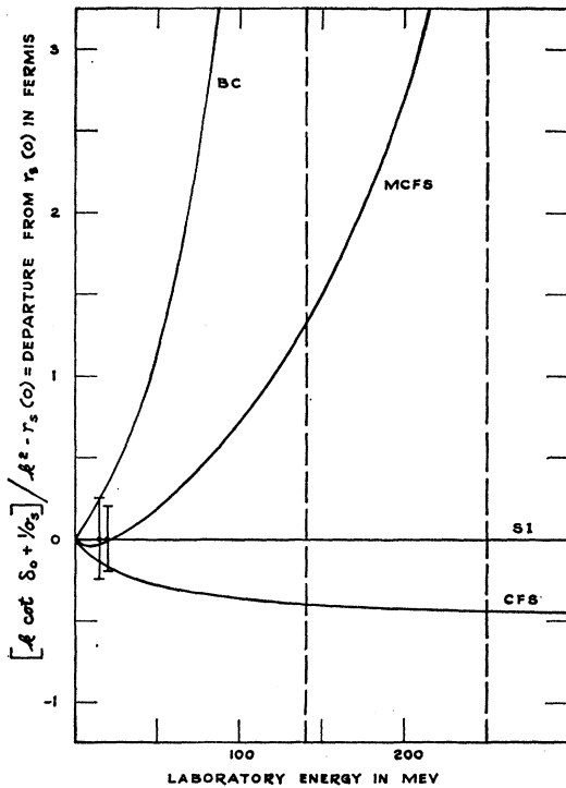
FIG. 1. Predictions for the effective range function defined by r_s(k^2) = 2(k \cot \delta_0 + 1/a_s)/k^2 . The expected behavior for models which have the long-range OPE interaction and sufficient parameters to fit a_s , r_s(0) , and the zero in \delta_0 at 250 MeV is given by the curve MCFS. The three other curves are CFS [Cini, Fubini, and Stanghellini (reference 42)], SI (shape-independent approximation), and BC [boundary condition (references 45, 46)].
