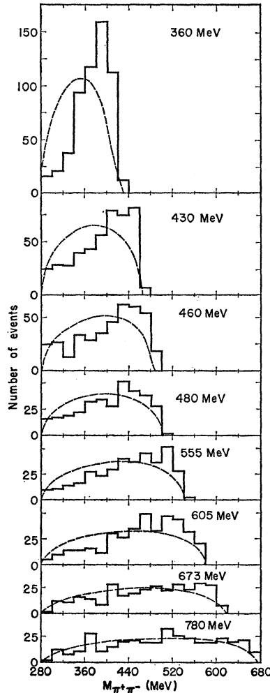
FIG. 3. \pi^+\pi^- effective-mass distribution at each beam energy. The dashed curves represent phase space.
