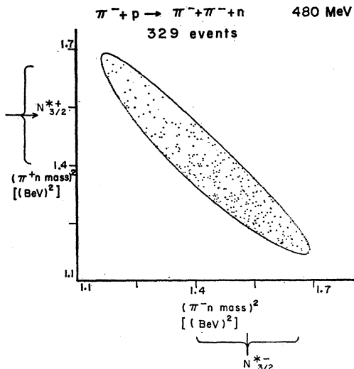
FIG. 2. Dalitz plot for reaction (1) at 480-MeV beam energy. The position and width of N^*(1238) are indicated in both charge states.
