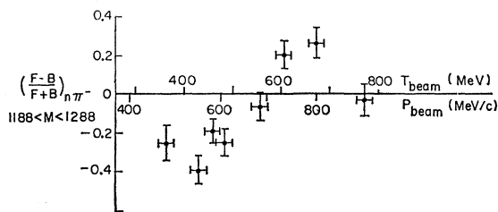
FIG. 5. The ratio (F-B)/(F+B) for events with 1188 \leq M_{\pi^-n} \leq 1288 . F stands for the number of events for which the \pi^-n system is produced forward in the reaction center-of-mass system, B for those produced backward.
