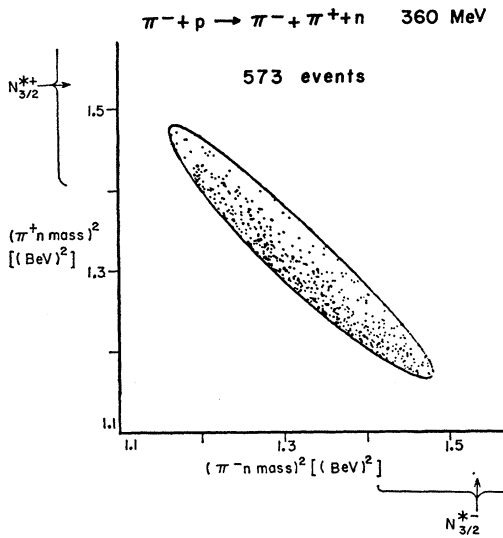
FIG. 1. Dalitz plot for reaction (1) at 360-MeV beam energy. The position and width of N^*(1238) are indicated in both charge states.
