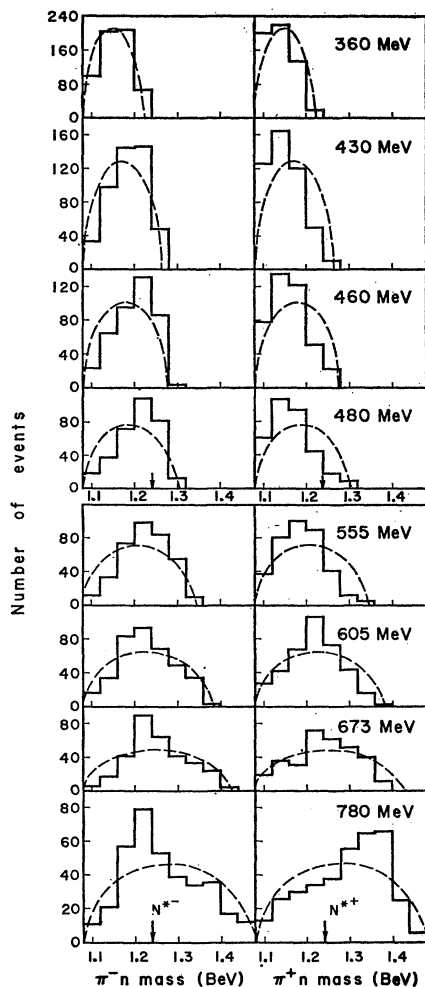
FIG. 4. \pi^+n and \pi^-n effective-mass distribution at each beam energy. The dashed curves represent phase space. The arrows point to the position of the N^* mass of 1238 MeV.
