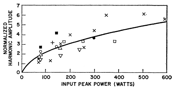
FIG. 6. The observed maximum harmonic output at 3.1^\circ\text{K} versus input rf power. The solid curve is drawn for the harmonic power proportional to P_{rf} .
