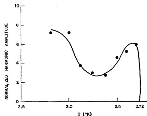
FIG. 8. The observed maximum harmonic output versus temperature. This curve is an average over all the data taken for all the pure bulk samples.
