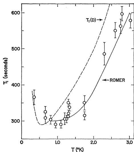
FIG. 4. The spin-lattice relaxation time T_1 in liquid \text{He}^3 at SVP: \circ —this research in a 3-mm quartz bulb; —, Romer (Ref. 3) in Pyrex bulbs, smoothed data; - - - - T_1(D) , derived from self-diffusion measurements (Ref. 7).
