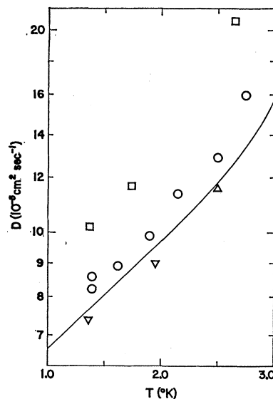
FIG. 5. The coefficient of self-diffusion D in liquid He 3 at SVP. Several different sample containers were used: \nabla —2.5-mm-i.d., 5-mm-long Delrin cylinder; \triangle —3-mm-i.d. quartz bulb; \circ —8-mm-i.d. Pyrex bulb; \square —10-mm-i.d. Pyrex bulb; the solid line represents the results of Hart and Wheatley (Ref. 7) obtained in a 7.6-mm-i.d., 8.4-mm-long epoxy resin cylinder.
