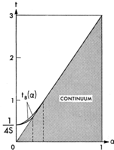
FIG. 5. Sketch of t_B(\alpha) for the three-dimensional lattice and \alpha_i = \alpha . The lower curve is doubly degenerate. Threshold values of \alpha are given by (77).
