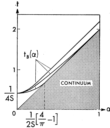
FIG. 6. Three-dimensional bound-state behavior for \alpha_1 = \alpha_2 = \alpha and \alpha_3 = 0 .
