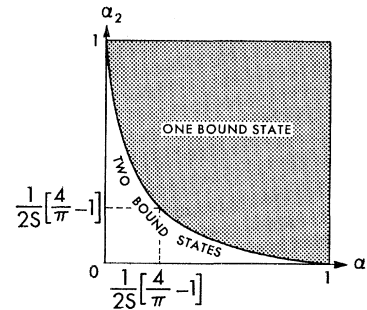
FIG. 4. Sketch of threshold for the appearance of the second bound state for each \mathbf{K} for the two-dimensional lattice \alpha_i = \cos \frac{1}{2} K_i .
