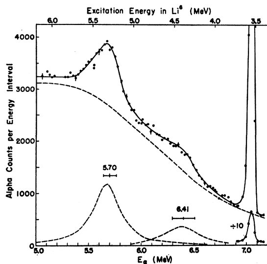
Fig. 2. Energy spectrum of the alpha particles from \text{Be}^9(p, \alpha)\text{Li}^6 at 30° laboratory angle, 10-MeV incident proton energy. The energy interval \Delta E is E/180 , but the observed number of alpha particles of energy E_\alpha has been divided by E_\alpha so that the spectrum shape corresponds to a constant energy interval. Alpha particles of 7-MeV energy lose 45 keV in passing through the beryllium foil target. The observed spectrum (solid line) has been decomposed into discrete groups and a residual continuous spectrum (dashed lines). The bars over the dashed curves indicate the alpha-particle energy, and the uncertainty in the energy, which leads to the excitation energy listed in Table I.
