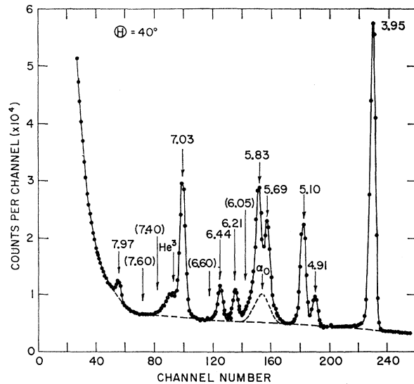
FIG. 1. Pulse-height spectrum of N^{14}+p observed at 40^\circ to the proton beam at a proton energy of 10.2 MeV. The proton peaks are labeled by the N^{14} excitation energy in MeV of the levels to which they are assigned. Unobserved peaks are indicated by arrows and excitation energies in parenthesis. The dashed curve shows the assumed course of the background including the \alpha group from the N^{14}(p,\alpha)C^{11} (ground state) reaction. The solid curve between channels 70 and 200 is a computer fit to the data (closed circles).
