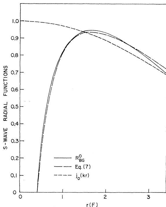
FIG. 2. The Bethe-Goldstone function (5), the function (7) with the parameters (8a), and the free-pair function j_0(kr) for c=0.4 F, k_F=1.36_6 F ^{-1} , and k=\mu^*k_F/2M_N^*=0.422 F ^{-1} .
