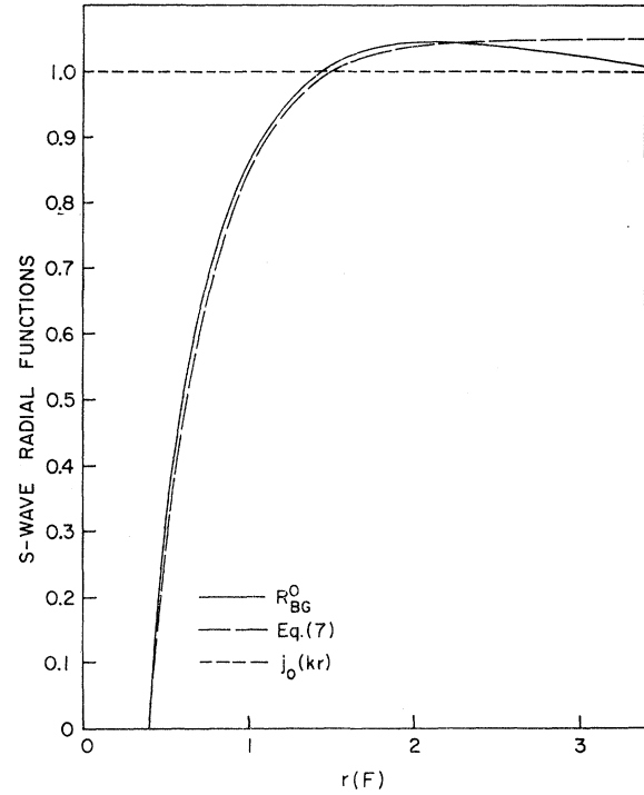
FIG. 1. The Bethe-Goldstone function (5), the function (7) with the parameters (8a), and the free-pair function j_0(kr) for c=0.4 F, k_F=1.36_6 F -1 , and k=0 .
