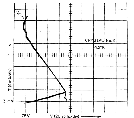
FIG. 2. Oscillograph of the current-voltage characteristic of CdS "tap" crystal No. 2 at 4.2°K. The values of V_t and V_m are, respectively, 145 V ( I=7 mA) and 75 V ( I=29 mA).
