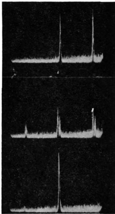
FIG. 8. Effect of polarizer on the 119 (left), 120, and 121 Mc/sec (right) beats between axial and higher TEM mn g modes of the planar He-Ne laser. Upper—polarizer at 0^\circ ; middle—polarizer at 45^\circ ; lower—polarizer at 90^\circ to vertical. Modes linearly polarized; stray transverse magnetic field at 4 Oe is present.
