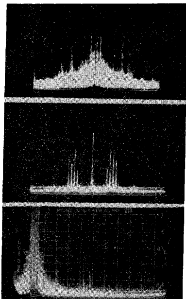
FIG. 6. Upper trace—noisy low-frequency beats due to stray transverse magnetic field of 4 Oe. Frequency sweep \pm 200 kc/sec. Middle trace—strong low-frequency beat phenomena between oppositely circularly polarized modes. Axial magnetic field 30 Oe, frequency sweep 50 kc/sec/cm. Lower trace—strong low-frequency beats and 1 Mc/sec beats between axial and transverse modes. Axial magnetic field 45 Oe. Frequency sweep 2 Mc/sec.
