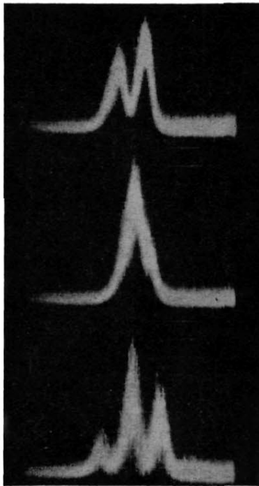
FIG. 14. Axial magnetic field—de-polarization effects in He-Ne laser. Upper—zero field, modes linearly polarized at +60^\circ and -30^\circ to vertical. Middle—magnetic field 14 Oe, polarizations still essentially linear. Lower—magnetic field 27 Oe—modes circularly polarized.
