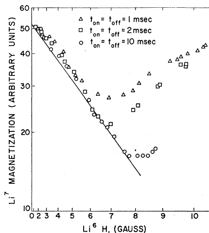
FIG. 4. \ln M_7 versus (H_1)_6^2 at 1.5^\circ\text{K} for N=22 , t_{\text{on}} = t_{\text{off}} = 1, 2, \text{ and } 10 msec, (H_1)_7 = 2.31 G. For this value of (H_1)_7 , (H_1)_6 = 6.1 G satisfies the Hahn condition. The solid line is calculated from Eqs. (28) and (34)
