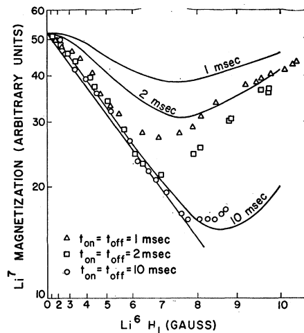
FIG. 9. \ln M_7 versus (H_1)^2 at 1.5°K. The solid curves are calculated using Eqs. (A9) and (A29). The solid straight line and data points are the same as in Fig. 4.
