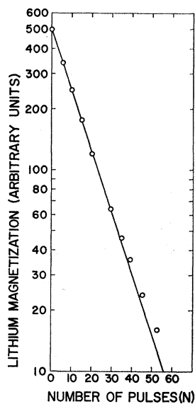
FIG. 8. \ln M_7 versus N at 1.5^\circ\text{K} in the completely demagnetized state [ (H_1)_7=0 ]. (H_1)_6=6.4 G, t_{\text{on}}=t_{\text{off}}=6 msec. The value of (H_1)_6 corresponds to the broad minimum in Fig. 7. The solid line is drawn to indicate the exponential dependence.
