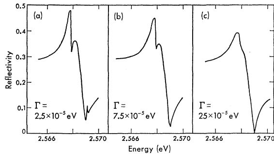
FIG. 4. The theoretical effects of increasing linewidth on 1s B series exciton spectrum for k \perp z , E \perp z . (a) \Gamma = 2.5 \times 10^{-5} eV, the peak at the longitudinal frequency is present at this small width; (b) \Gamma = 7.5 \times 10^{-5} eV; (c) \Gamma = 25 \times 10^{-5} eV, the extra structure is being washed out at increased linewidth.
