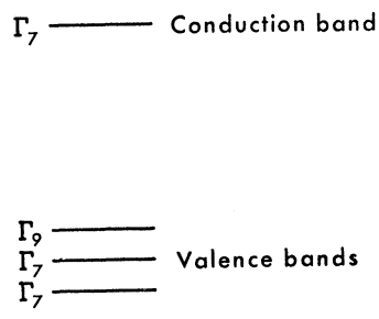
FIG. 1. The symmetries of the conduction band and the three principle valence bands of wurtzite crystals, such as CdS.
