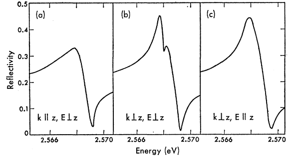
FIG. 2. The reflection spectra of the 1s B series exciton in a single sample of CdS from Hopfield and Thomas. (a) k \parallel z , E \perp z , (b) k \perp z , E \perp z , (c) k \perp z , E \parallel z ; only (b) shows effect.
