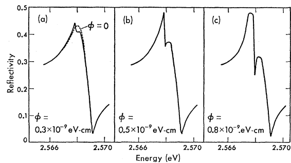
FIG. 5. The theoretical effect of increased linear splitting on the reflectivity spectrum. (a) \phi = 0 (dashed line) and \phi = 0.3 \times 10^{-9} eV-cm (solid line); (b) \phi = 0.5 \times 10^{-9} eV-cm; (c) \phi = 0.8 \times 10^{-9} eV-cm. The middle value appears as the most reasonable fit to the experimental data, Fig. 2.
