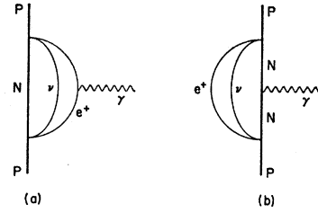
FIG. 3. Diagrams contributing to the electric-dipole moment of a proton in the absence of W mesons.
