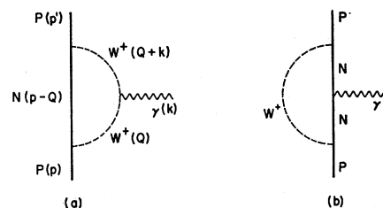
FIG. 1. Diagrams contributing to electric-dipole moment of a proton assuming the existence of intermediate weak vector bosons ( W ).
