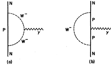
FIG. 2. Diagrams contributing to electric-dipole moment of a neutron assuming the existence of intermediate weak vector bosons.
