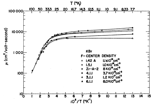
Fig. 2. Electronic Hall mobility in KBr as a function of reciprocal temperature for crystals of different F -center density.
