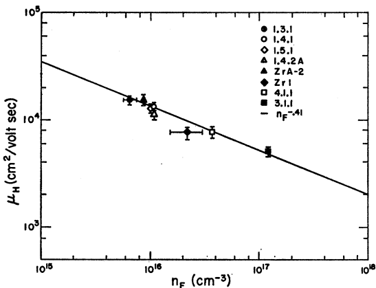
FIG. 4. The Hall mobility in KBr at T = 7.7^\circ\text{K} as a function of F -center concentration. The solid line is a plot of the function \mu_H n_F^{-0.41} where A is a constant.
