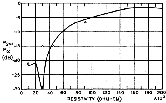
FIG. 1. \frac{P_{2\omega}}{P_{\omega}} = P_{\omega} \left[ \frac{1}{8V_0c} \left( \frac{c_{III} e^{-1}}{c} \right)^2 \sin^2 \left[ \frac{(\omega X/V_0)(V_{2\omega} - V_{\omega})}{V_0} \right] \right] at 30 Mc for P_{\omega} = 0.18 \text{ W/cm}^2 as a function of sample resistivity on 7-mm crystal.
